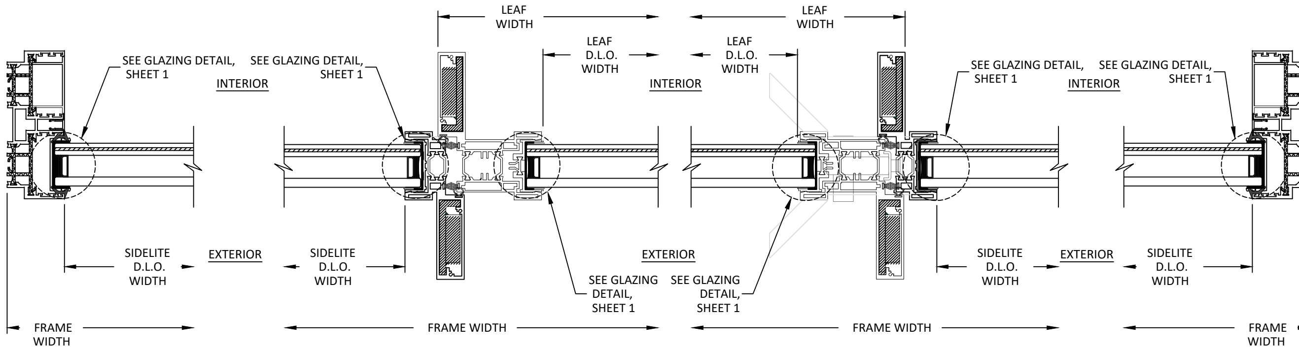
D 8 VERTICAL SECTION SIDELITE JAMB
