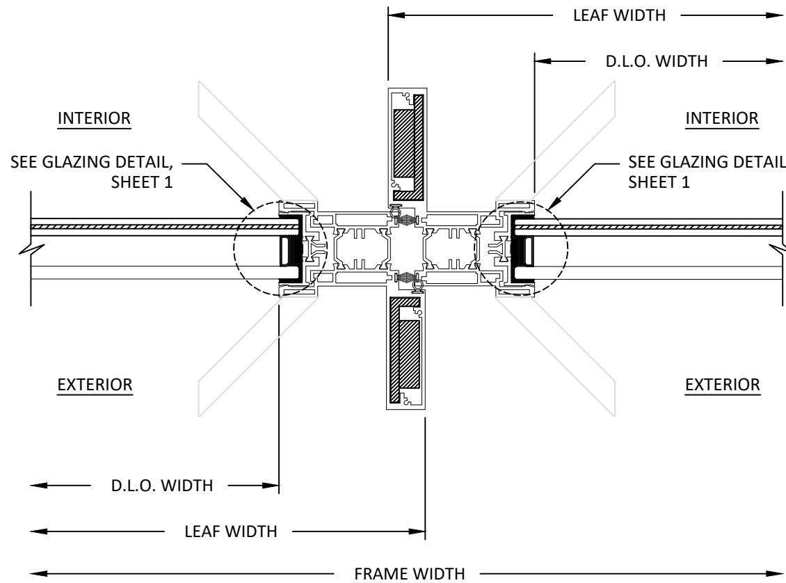
B 8 VERTICAL SECTION MEETING STILE
